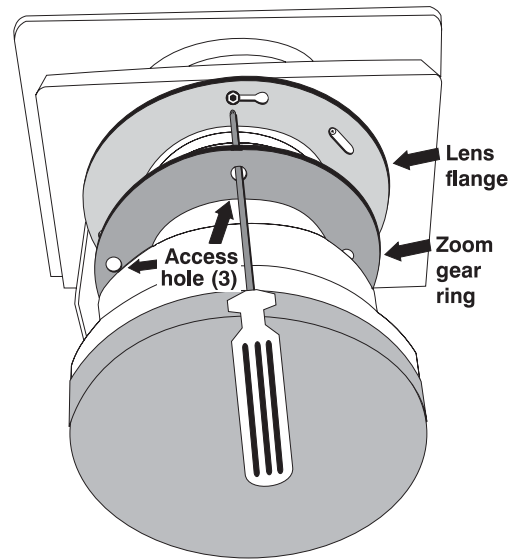
Align zoom gear ring to access 3 screws -ZOOM LENS-
