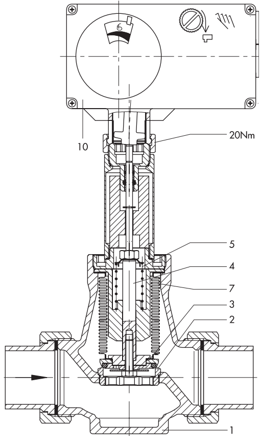
Type 3222/5724 Special version for temperatures up to 200 °C and with plug balanced by a bellows
