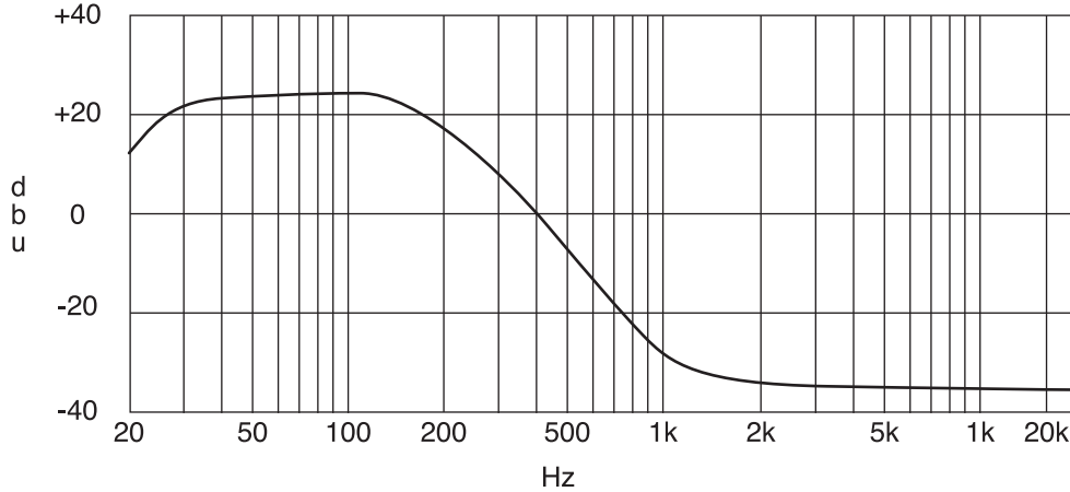
Resolv sub88 Frequency Response / Bande passante des Resolv sub88 / Resolv sub88 Frequenzgang Respuesta de frecuencia del Resolv sub88 / Risposta in Frequenza del Resolv sub88
