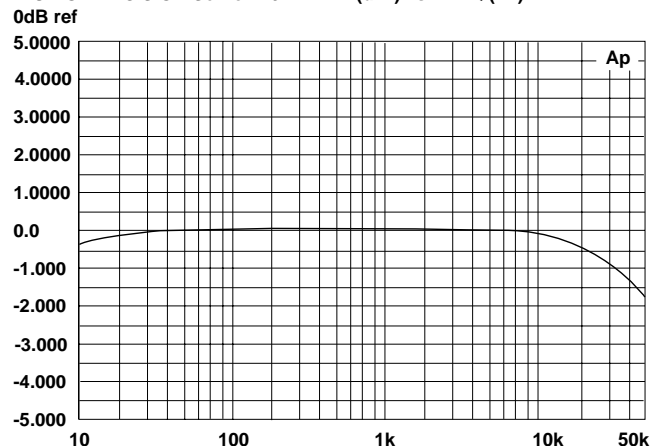
AUDIO PRECISION Servo 120 LEVEL (dBr) vs FREQ (Hz)
