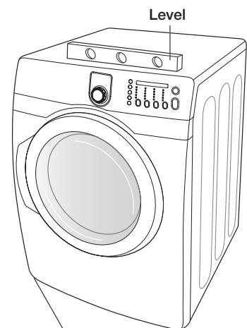
Leveling feet
