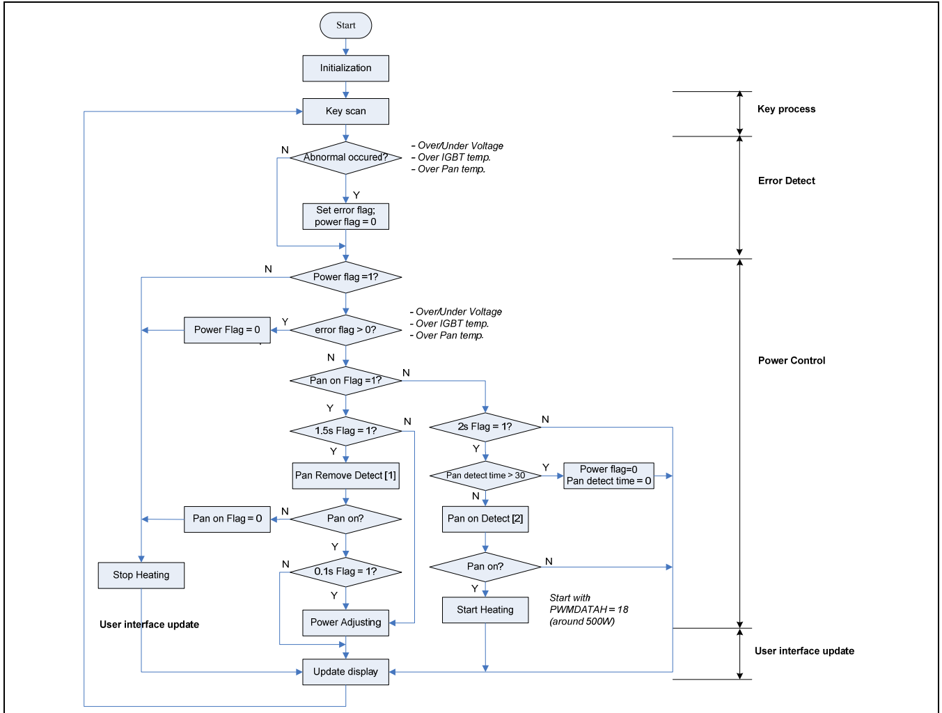
Figure 3-2 Software Diagram
