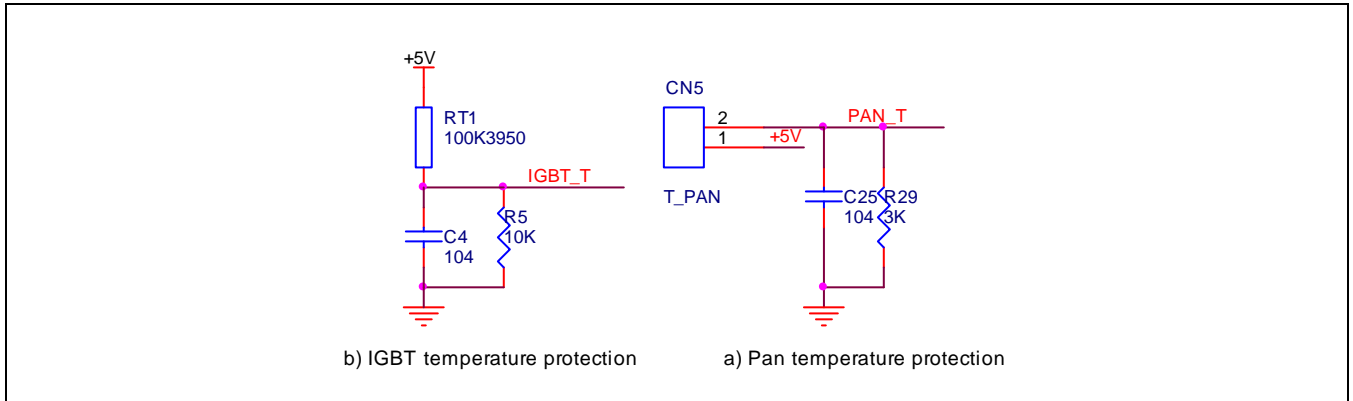
Figure 2-7 Over-Temperature Protection
