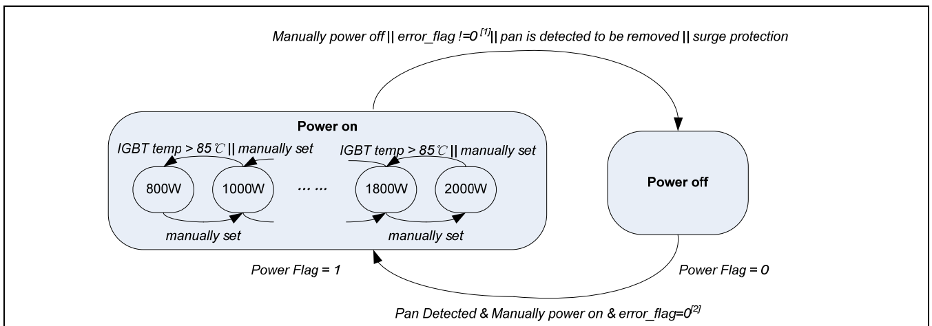
Figure 3-1 State Transition Diagram
