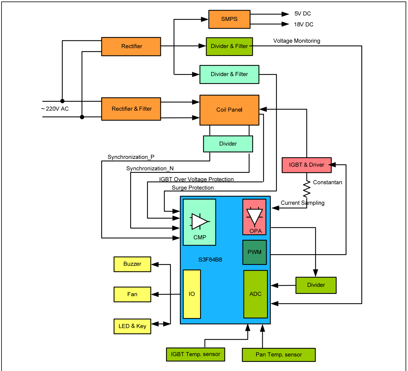
Figure 2-1 Block Diagram of IH Cooker System
