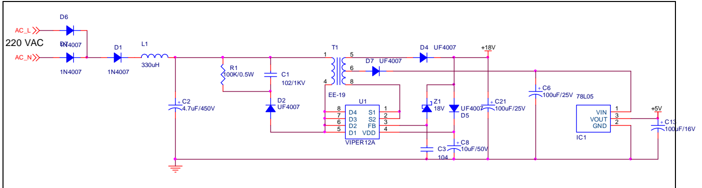
Figure 2-2 Power Supply Circuit
