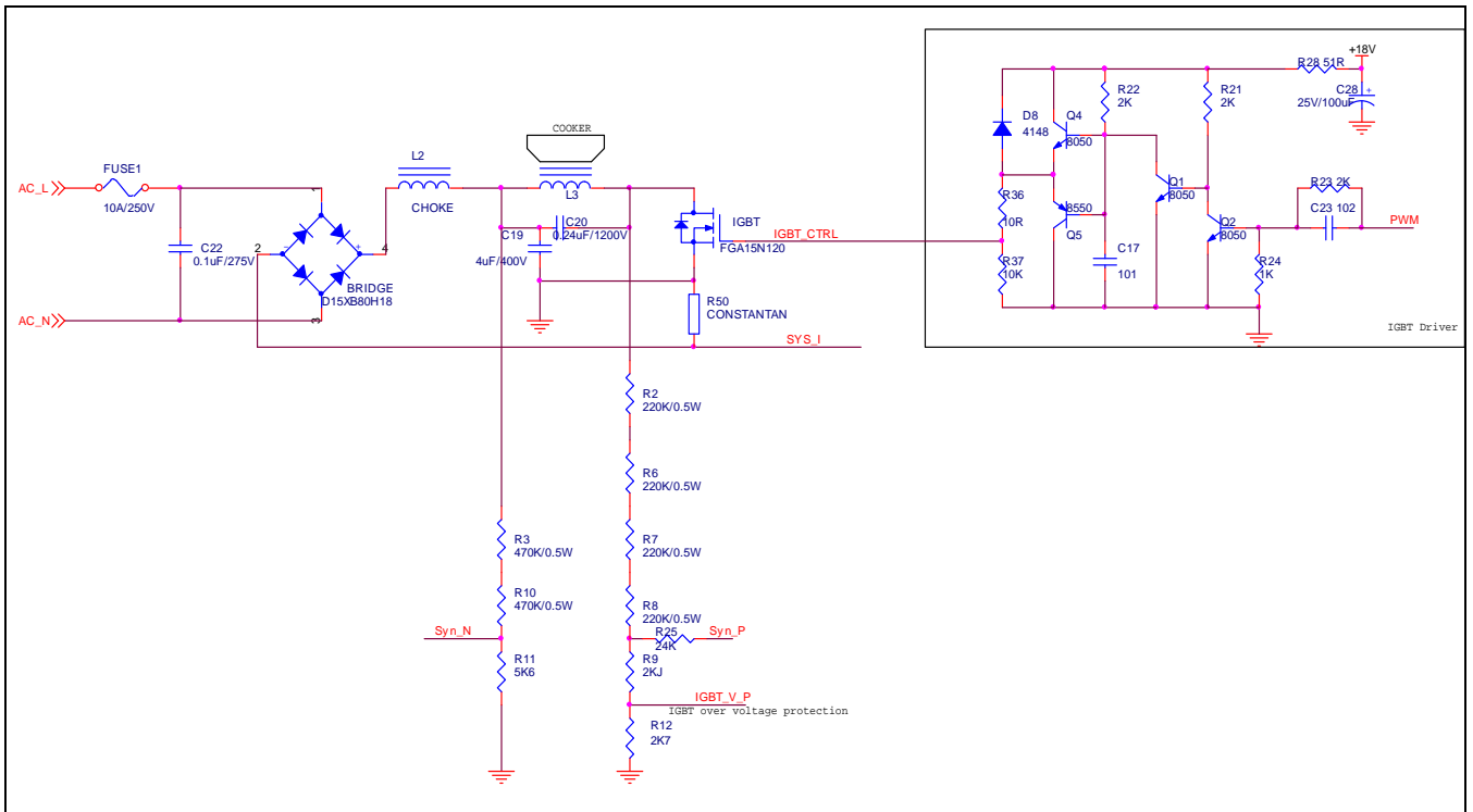
Figure 2-3 Power Supply Circuit
