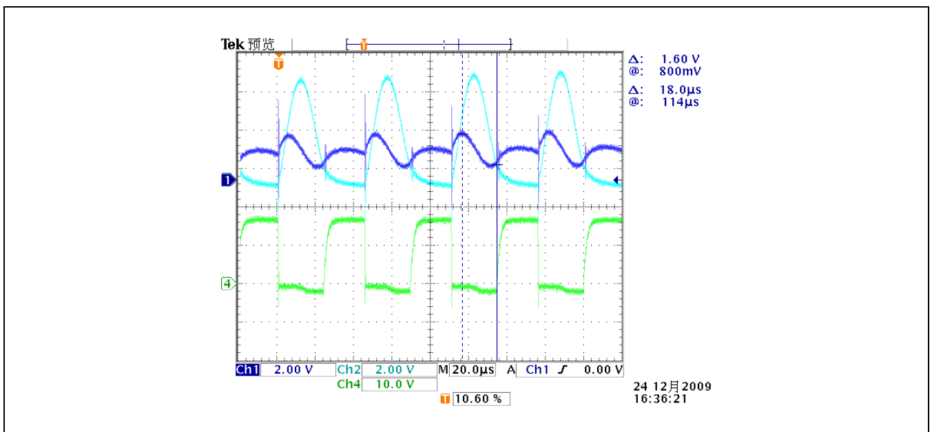
Figure 2-4 Waveform of the Synchronization Circuit
