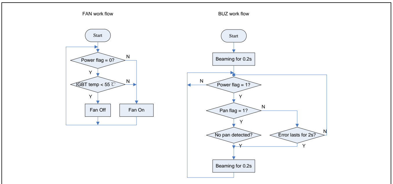
Figure 3-4 Fan and BUZ Workflow
