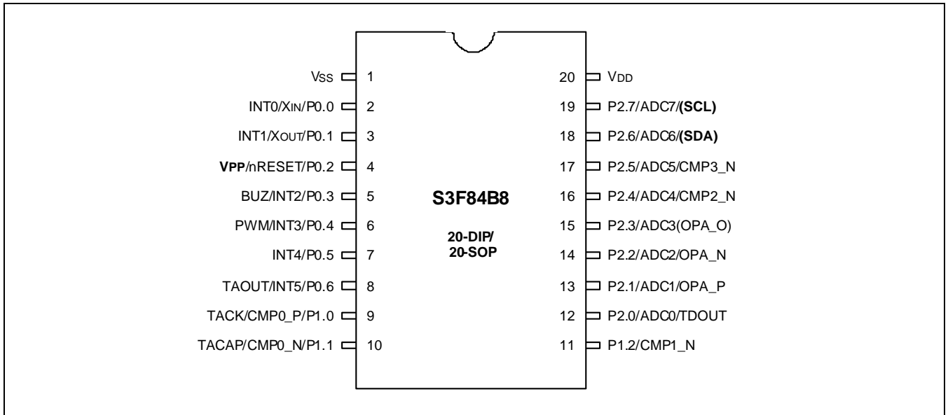
Figure 1-2 Pin Assignment in S3F84B8
