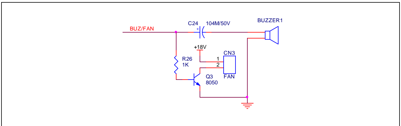
Figure 2-8 Buzzer and Fan Control
