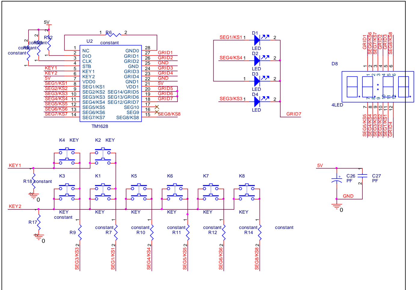
Figure 2-9 Key and Display Circuit
