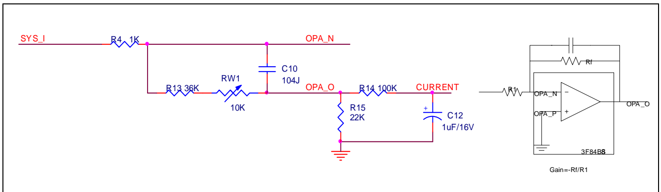
Figure 2-6 Current Measurement Circuit
