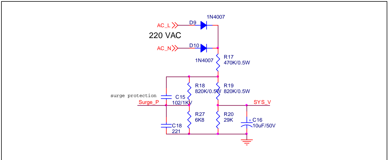
Figure 2-5 Voltage Measurement and Surge Protection Circuit
