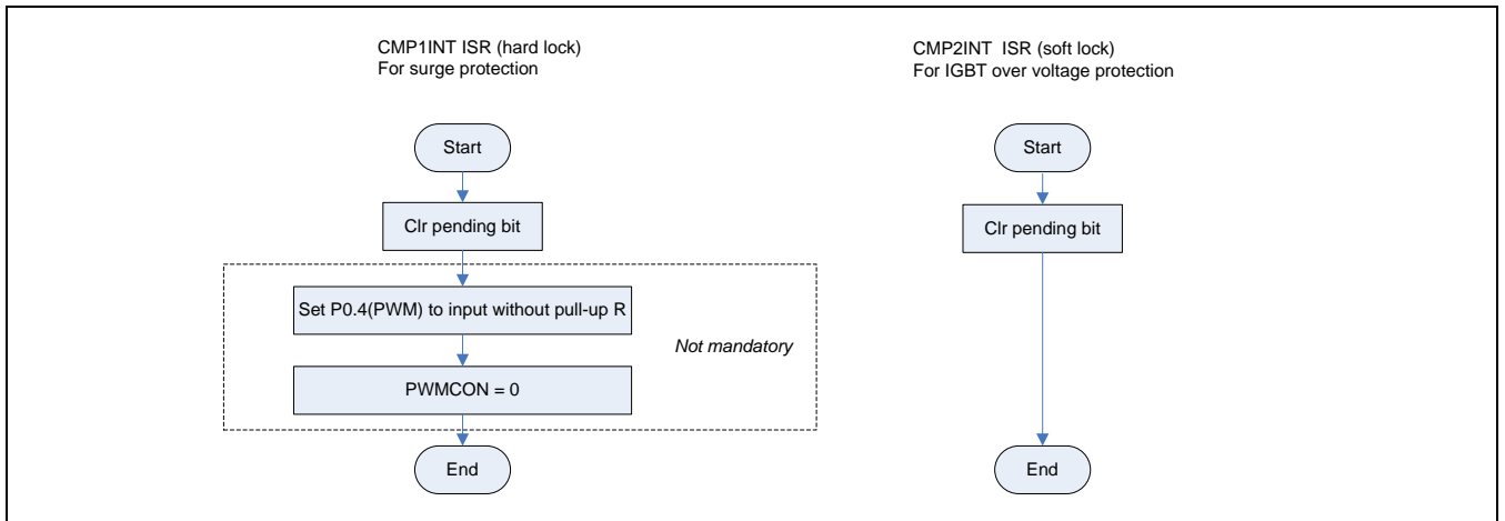
Figure 3-3 Interrupt Service Routine Diagram
