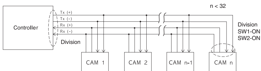
<RS-422A/RS-485 Full Duplex Organization>
