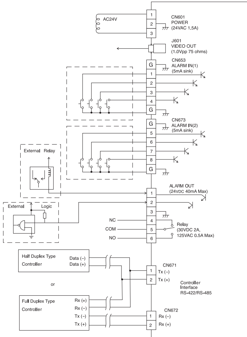
SCC-C6407 Adapter BOARD
