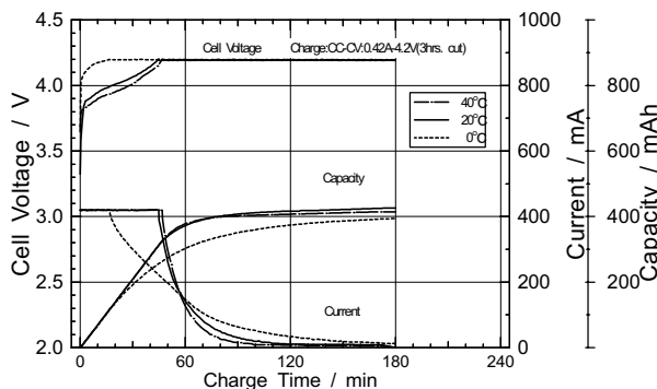
Charge characteristics
