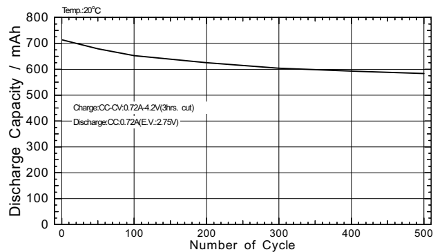
Cycle characteristics
