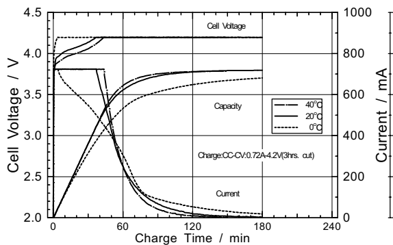
Charge characteristics
