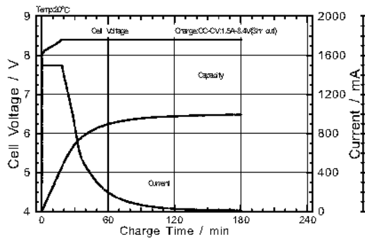
Charge characteristics
