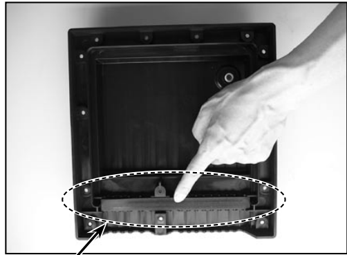
GASKET IN THE TERMINAL COVER
