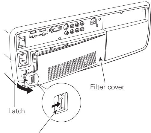
Press the latch and take off the filter covers.
