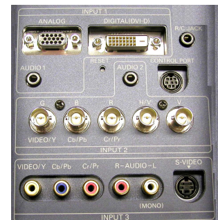
PLV-80/75 Input Panel
