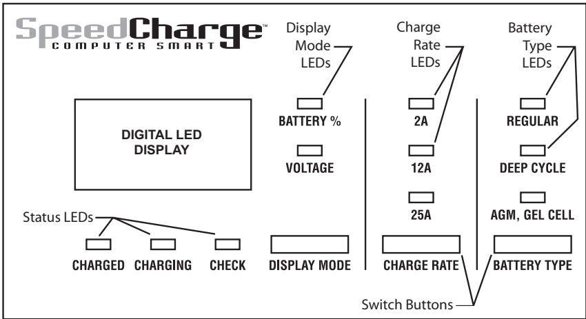
SCF-2500A CONTROL PANEL
