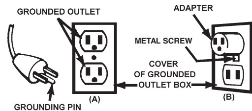
Grounding methods
