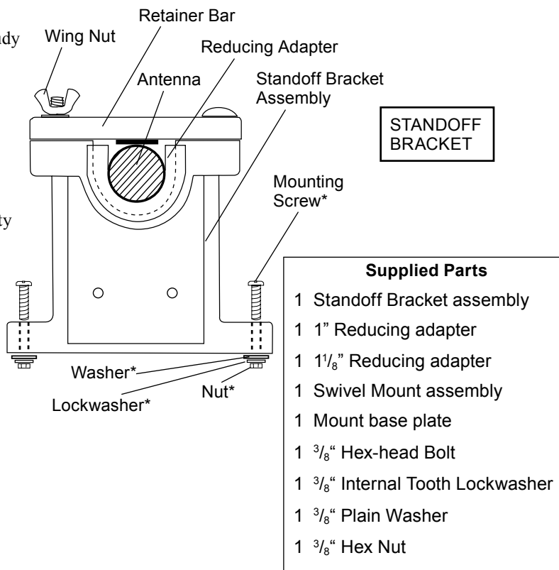
Bulkhead Mounting: SIDE VIEW
