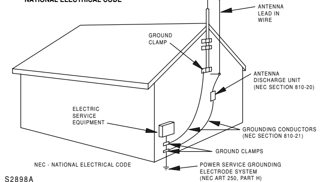
FIGURE A EXAMPLE OF ANTENNA GROUNDING AS PER NATIONAL ELECTRICAL CODE
