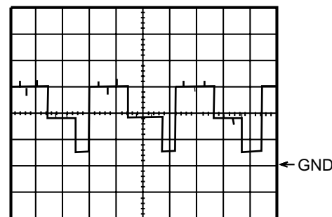
WF4 1DIV: 2V 20μsec Q 1521 Base
