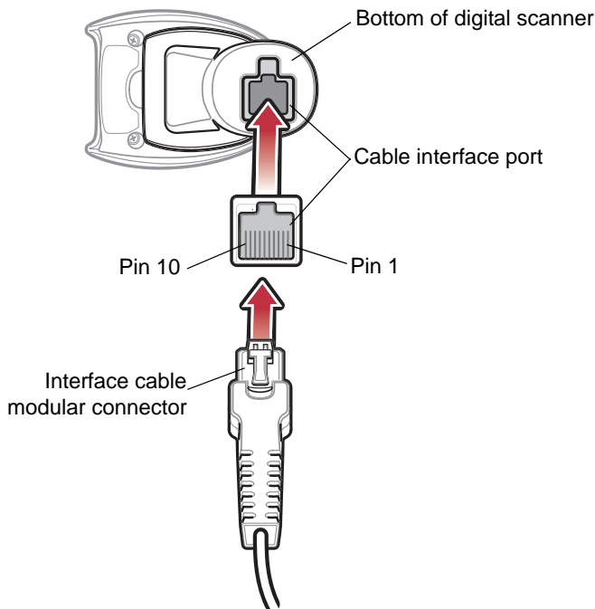
Figure 3-1 Digital Scanner Cable Pinouts
