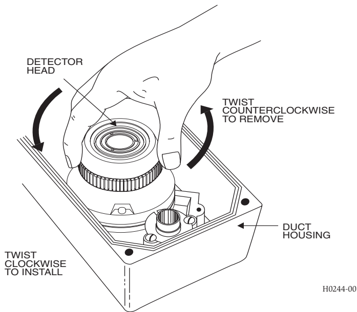
Figure 8. Detector head removal:
