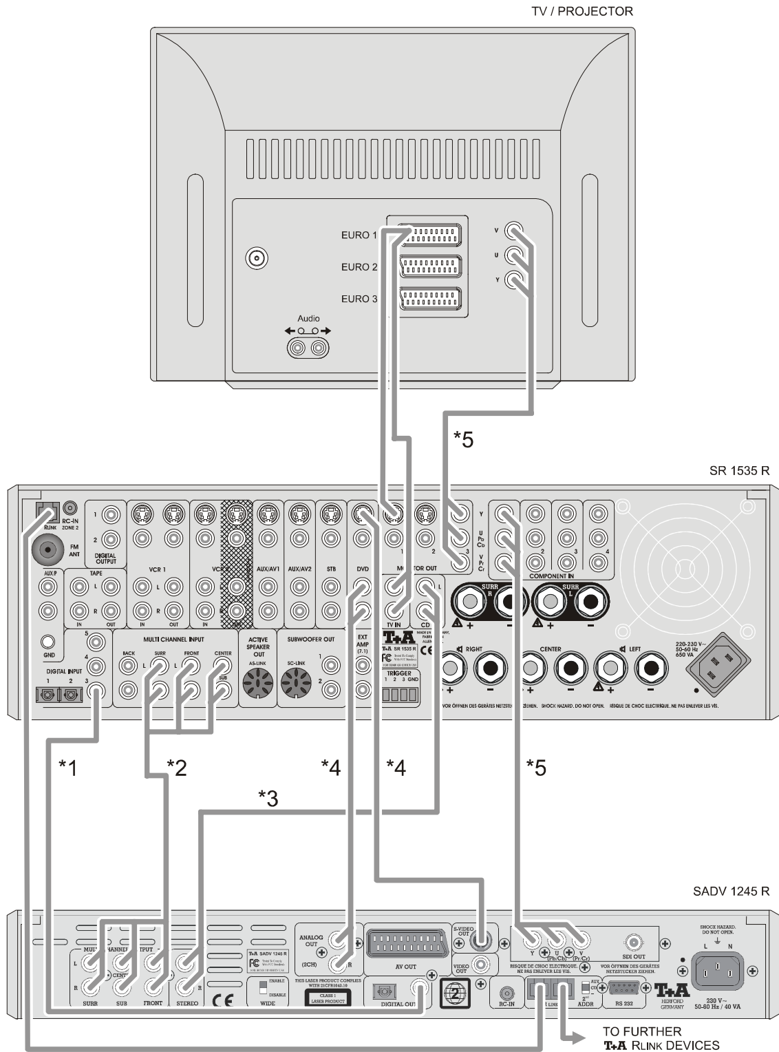
Wiring diagram 1: SADV 1245 R and SR 1535 R with S-Video and Component YUV Video
