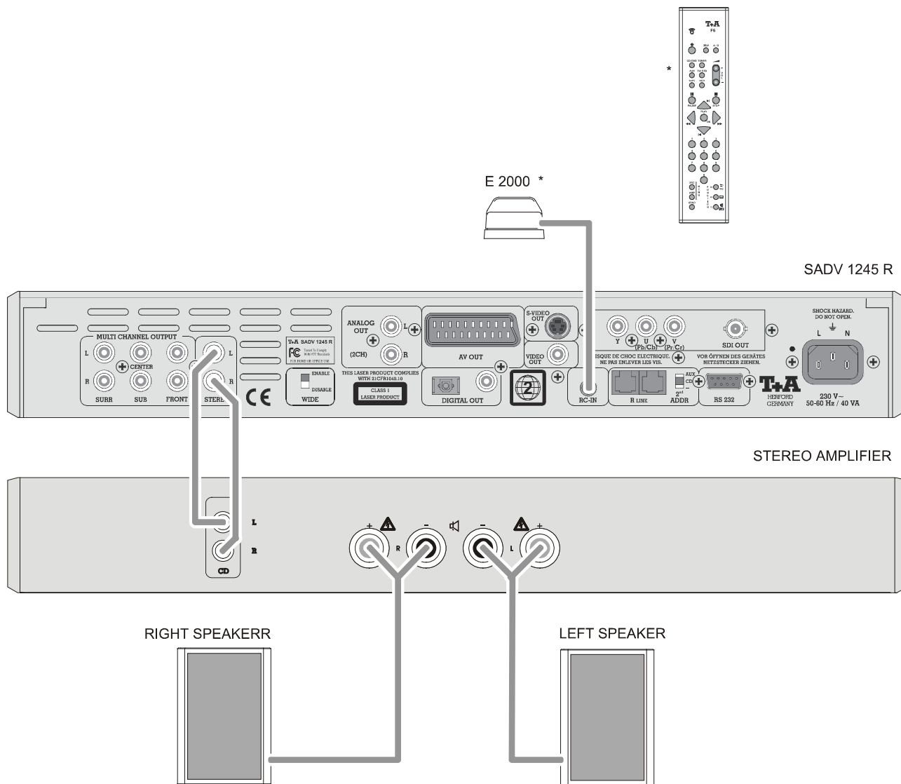
Wiring diagram 3: SADV 1245 R connected to a stereo amplifier
