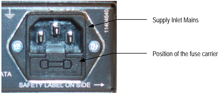
Figure 2.2: AC Power Inlet Assembly
