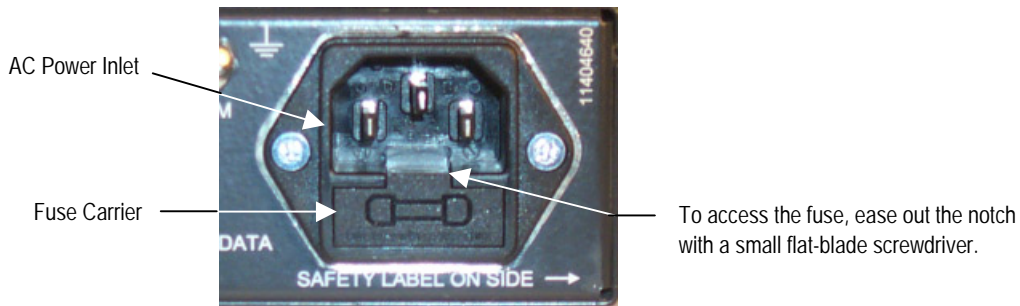
Figure 6.2: Fuse Carrier
