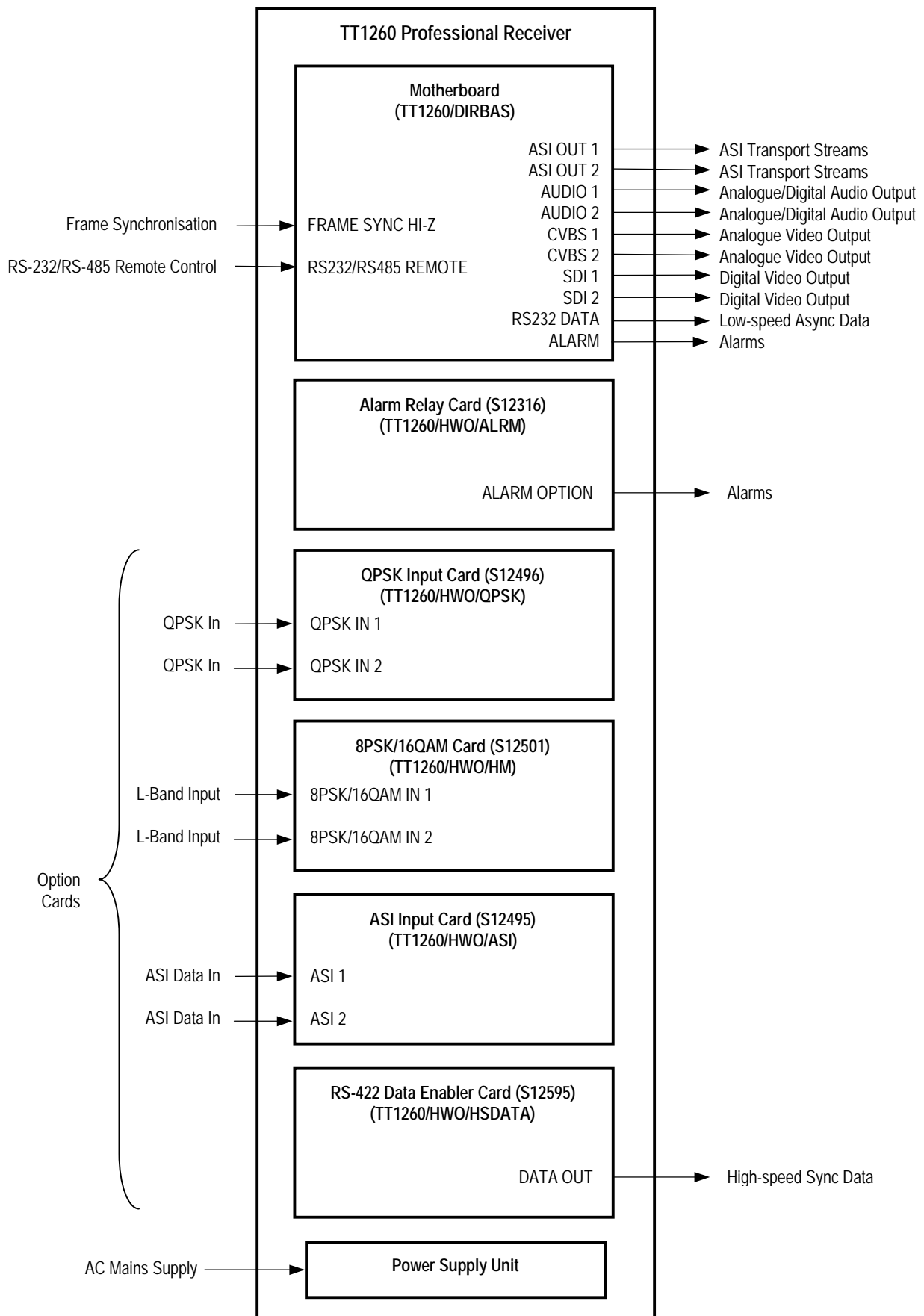
Figure 2.5: TT1260 Signal Connections
