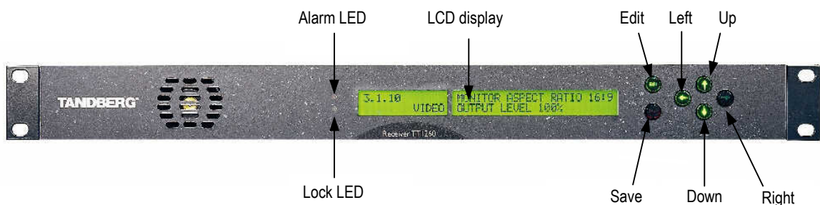
Figure 1.9: Front Panel Controls
