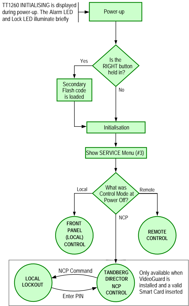
Figure 3.1: Power-up Operating Mode
