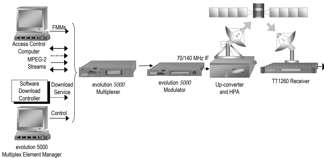
Figure 1.5: Typical Download Transmission System
