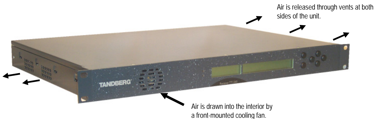
Figure 2.1: Air flow Through the Equipment
