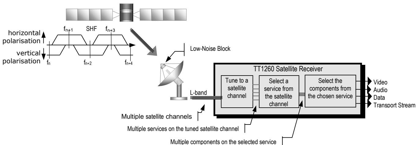
Figure 1.4: What the Satellite Receiver Does
