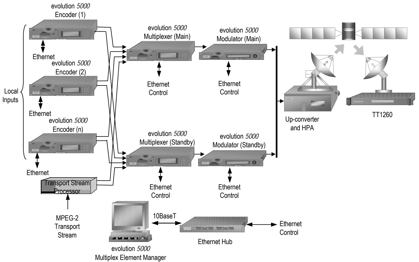
Figure 1.3: Typical Satellite Compression System
