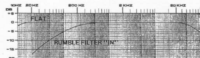
Rumble Filter
