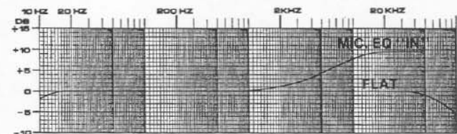
Microphone Equalization
