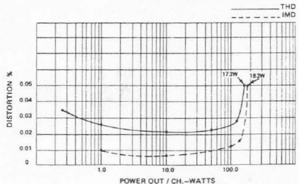
Tapco CP500M: Distortion vs. power output, into 8-ohm loads, both channels driven.
