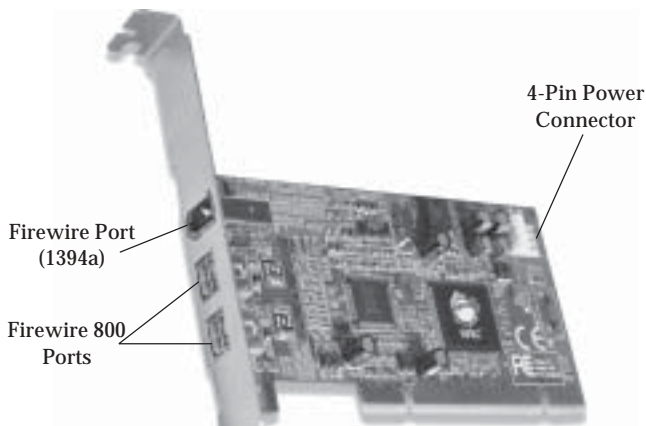
Figure 1. Board Layout
