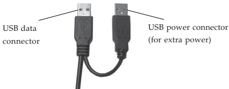
Figure 2: USB cable
