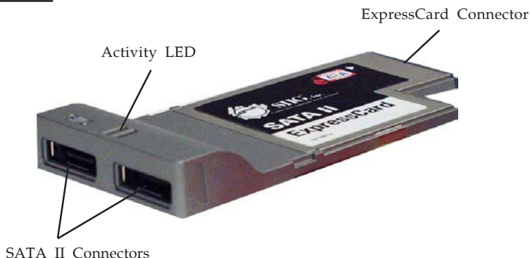
Figure 1. eSATA II ExpressCard RAID
