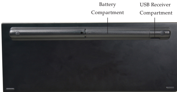
Figure 2: Rear Layout
