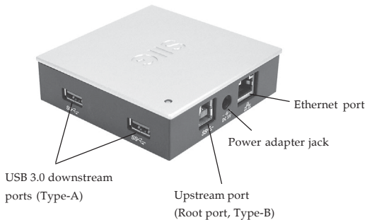
Figure 2: Rear Layout
