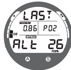
Fig. 19B - Last Alternate (Nitrox only)
