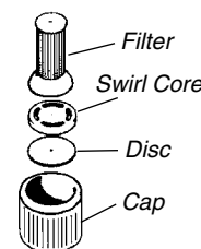
Cone Nozzle
