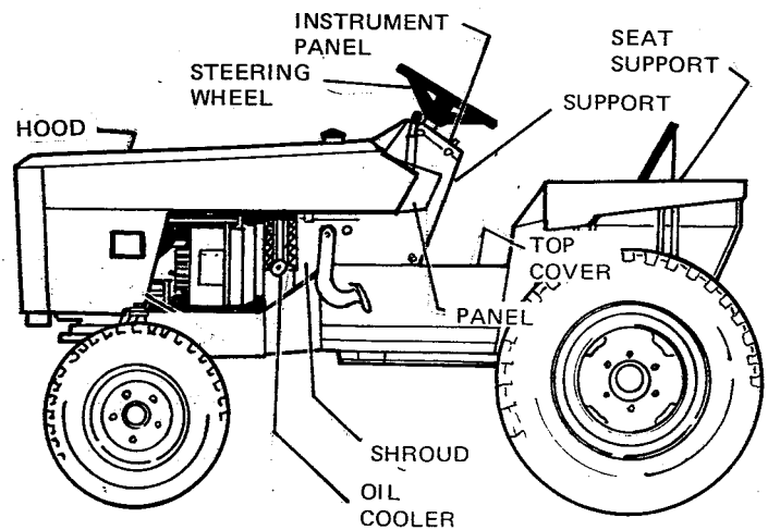
Figure 4. Tractor Components
