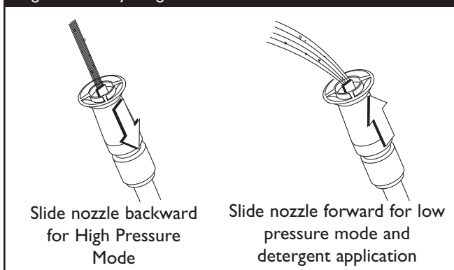
Figure 9 — Adjusting Nozzle for Pressure
