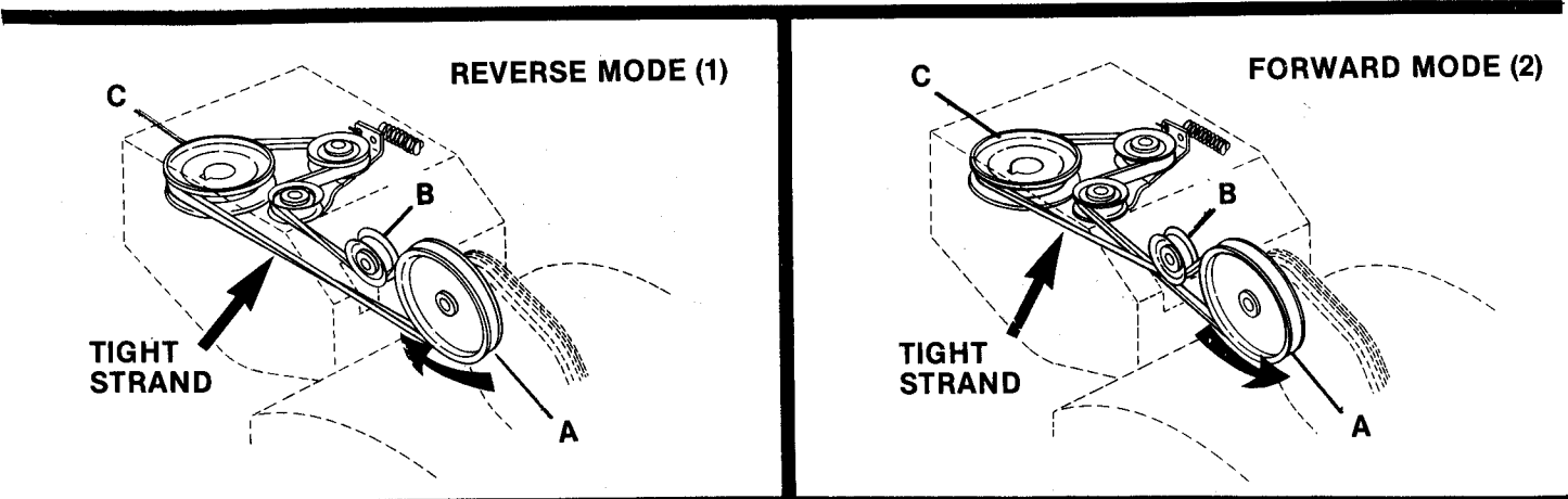
FIGURE 8 — TINE ROTATION BELT CHANGES
