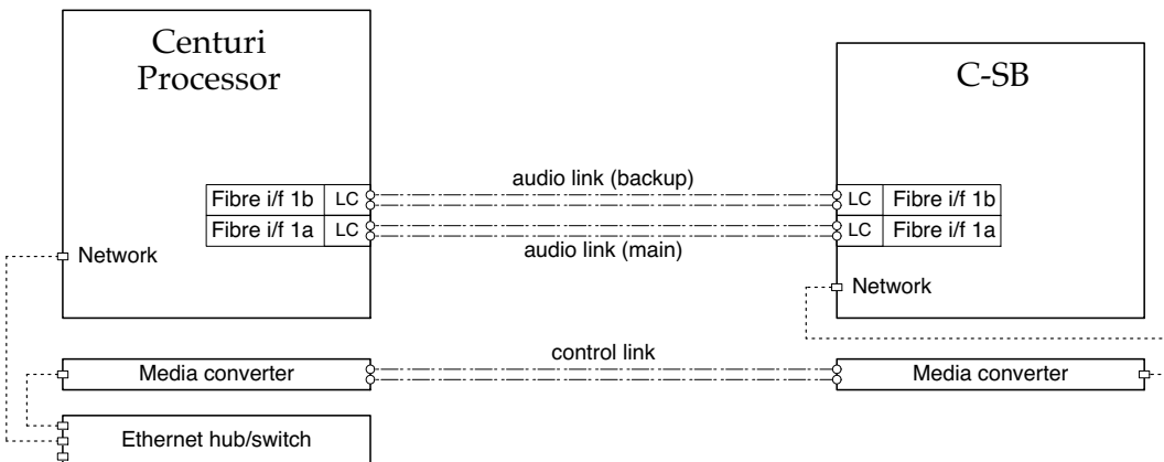
Dual Fibre-Link with fibre control link (>100m)
