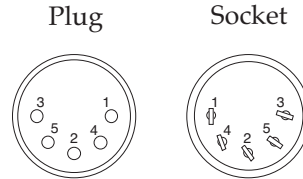
Connectors Viewed From Wiring Side
