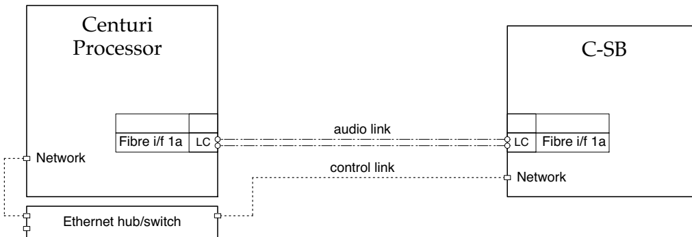
Single Fibre-Link with RJ45 control link (100m max)
