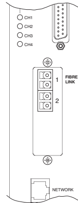
C-SB CPU Card With redundant Fibre Link
