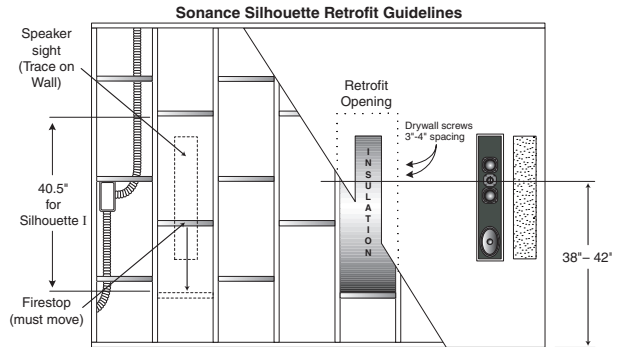
Figure 8: Retrofit construction for Sonance Silhouette speakers.
