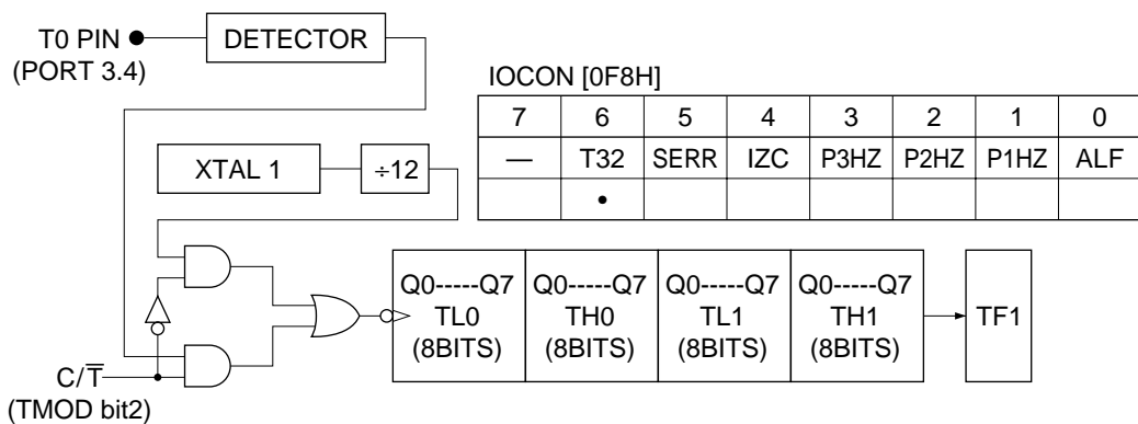
Figure 4-18 32-bit timer/counter
