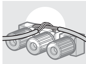
Stripped cords are touching each other due to excessive removal of insulation.
