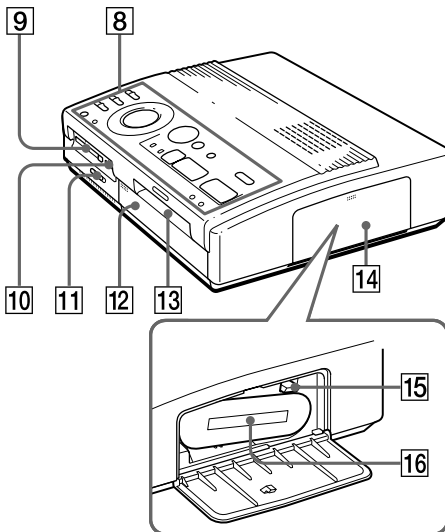
Cartridge compartment
