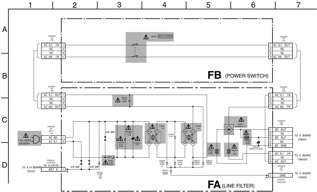
FA [ LINE FILTER ] FB [ POWER SWITCH ]
