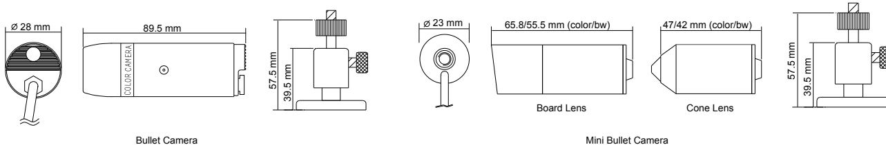
Bullet Camera
