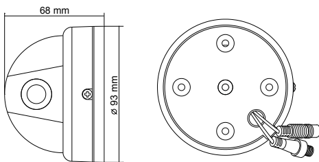
Vandal-proof
