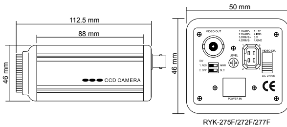
RYK-275F/272F/277F
