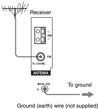
Outdoor FM antenna (aerial)
