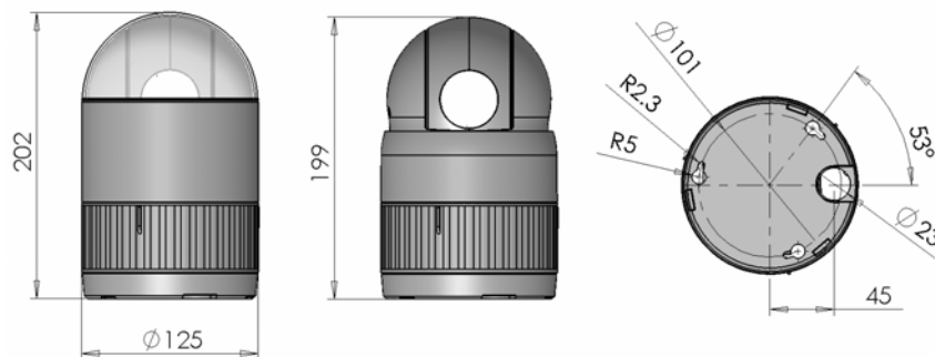
Figure 10– Dimension
