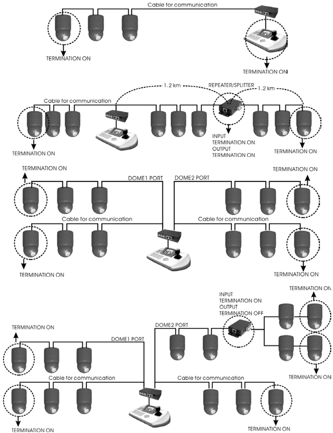
Figure 7- Termination Diagram
