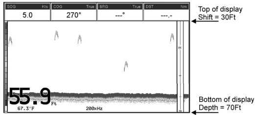
Figure 17.8.2 - Example of Depth and Shift
