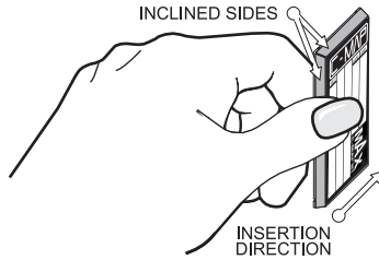
Figure 5.0 - Inserting C-CARD
