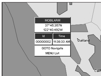
Figure 16.3.0b - Example of PTX warning window on CP180
