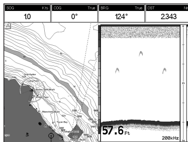
Figure 17.2.3 - Fish/Chart Page
