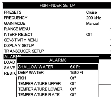
Figure 17.13 - Alarms menu
