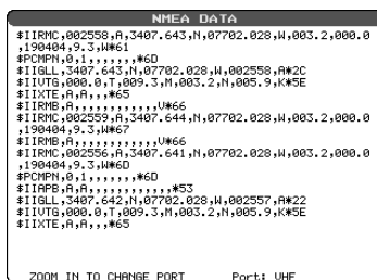
Figure 12.7a - NMEA Data page
