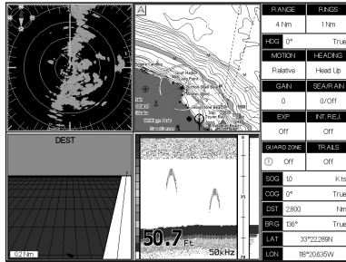
Figure 17.2.4.1 - Radar Combo Page
