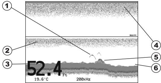
Figure 17.1.1 - The Fish Finder display
