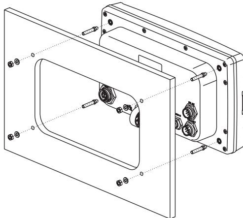
Figure 2.2a - Example of Flush installation CPF300i
