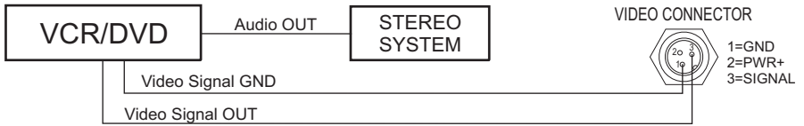
Figure 2.11.1 - VCR/DVD Input
