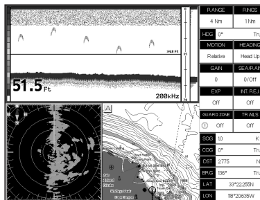
Figure 17.2.4.0 - Fish/Radar/Chart Page
