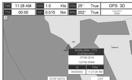
Figure 16.4.1c - Example of Stop Goto PTX on CP300
