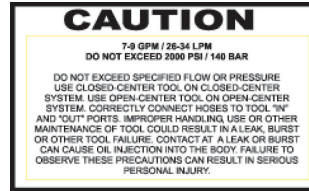
03786 7-9 GPM Decal
