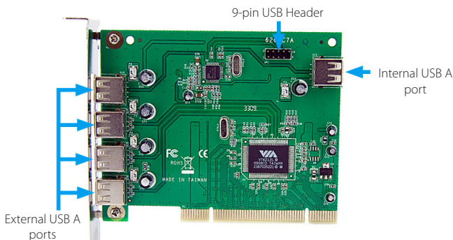
USB Pin-header Assignment on PCI Card
