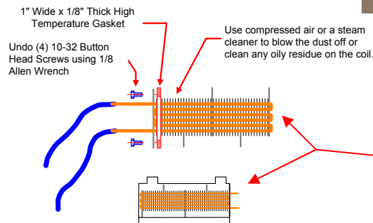
(Cooling Coil)
