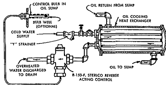
HEAT EXCHANGER
