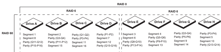
RAID 60 Example
