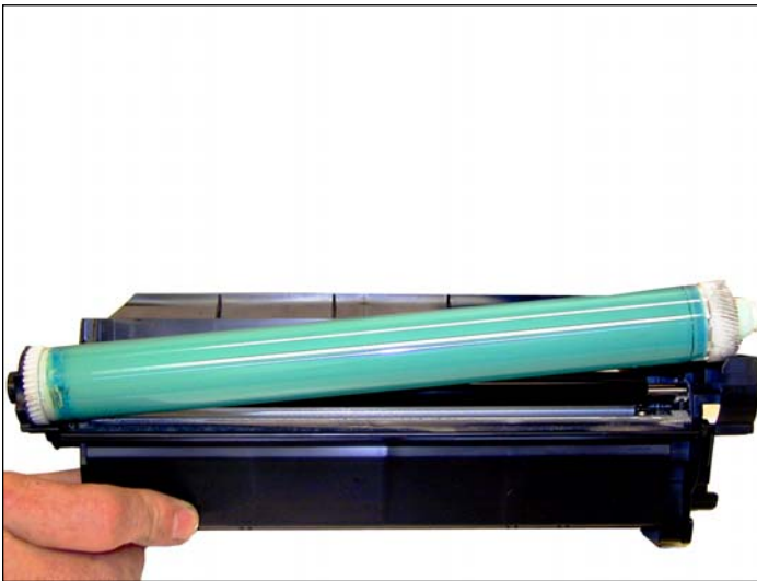
19. Install the drum small gear side first onto the drum axle pin
