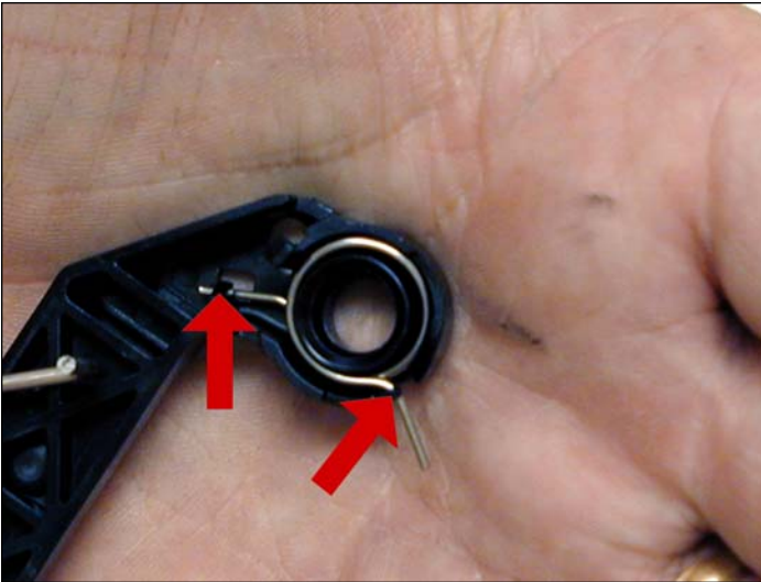
42. Install the spring into the drum cover arm as shown. Pull the upper tail of the spring until it fits into the notch in the arm hub.
