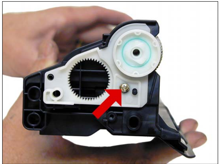
9. On the large gear side of the waste chamber, remove the screw and white plastic drum bushing.
