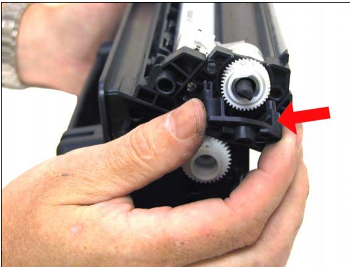
21. On the supply chamber, carefully pry off the Magnetic roller (MRS) cover, and remove.
