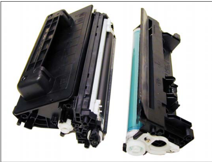
8. Separate the toner hopper and waste chamber.
