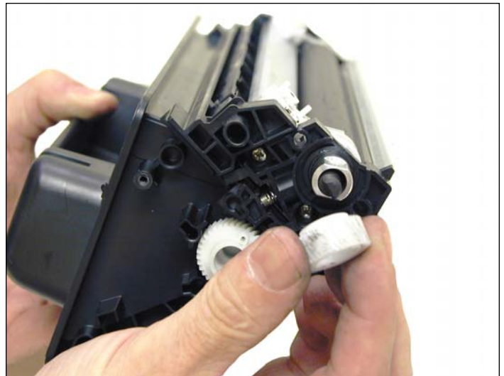
22. Remove the MRS drive gear.
