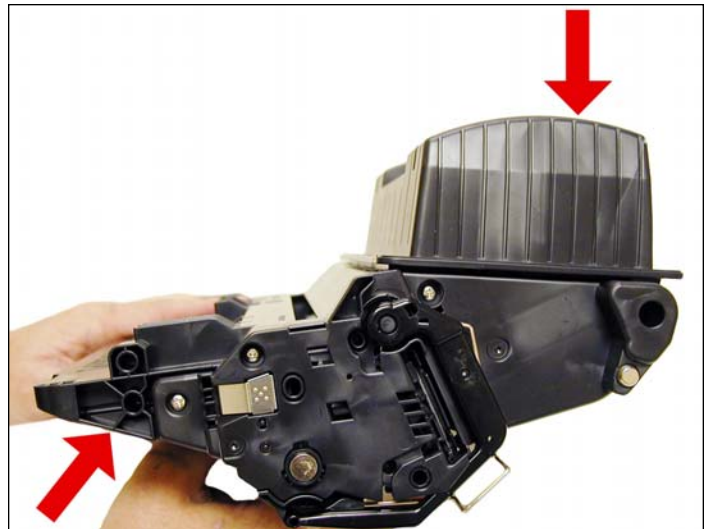
Left side of 64X
