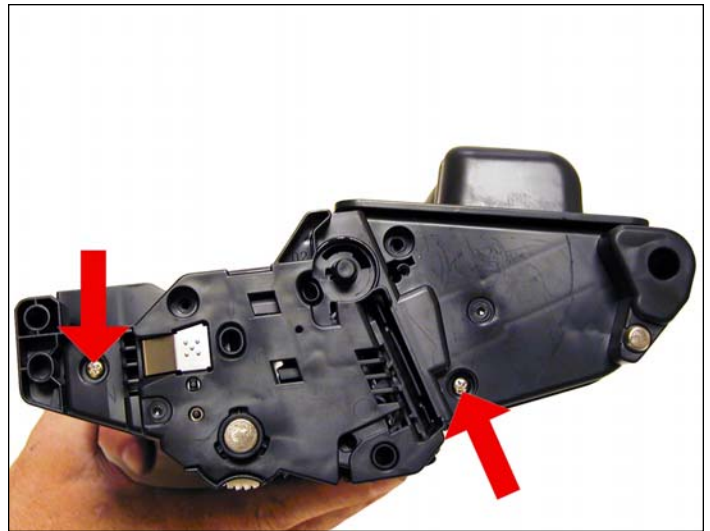
39. Hold the two sections of the cartridge together, and install the left (Contact side) end cap. Install a screw in the waste and supply sections to hold everything together.
