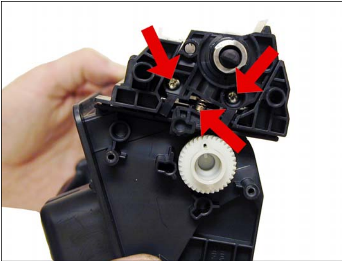
23. Note the location of the spring that sits between the MRS holder and the hopper.
