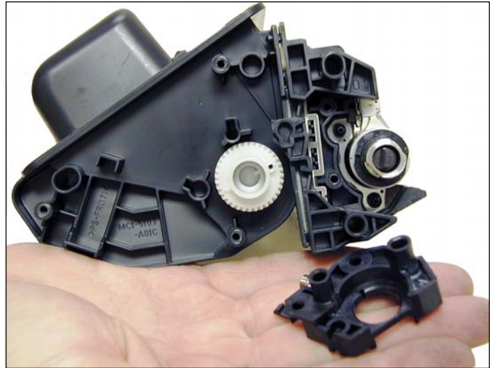
Remove the two screws, spring and the holder.
