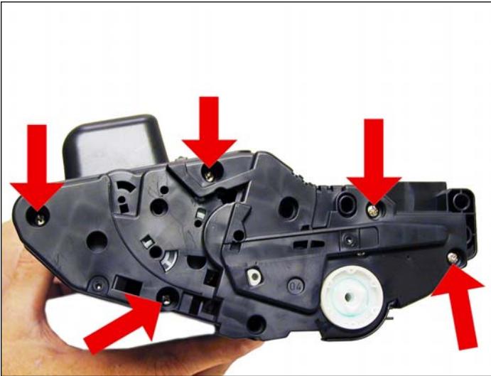
40. Install the right side end cap and five screws.
