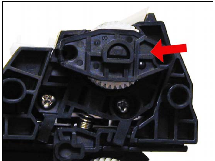
37. Install the keyed MRS cover. Make sure that the keyed hole in the cover matches the keyed end of the magnet in the MRS assembly.
