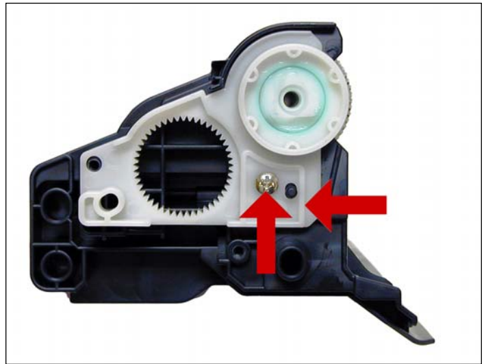
20. Install the white plastic drum bushing and screw. If the OEM drum grease is dirty, clean it off with alcohol, and replace with white lithium grease.
