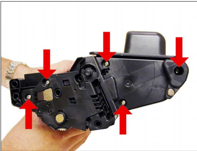
6. Remove the five screws from the left end cap.
