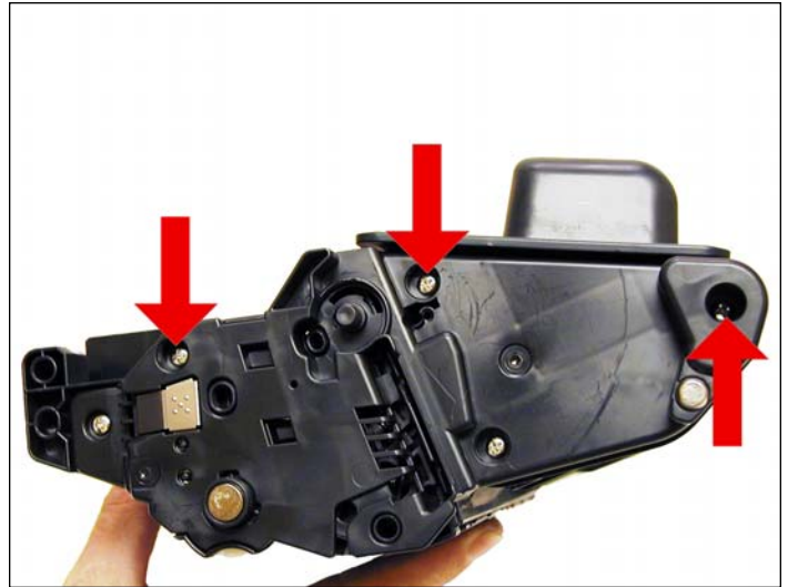
41. Install the remaining three screws on the left end cap.
