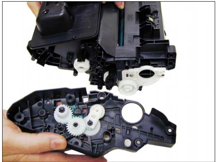
7. Remove the right and left side end caps from the cartridge. Note that the gears do not come off the gear (right) end cap.
