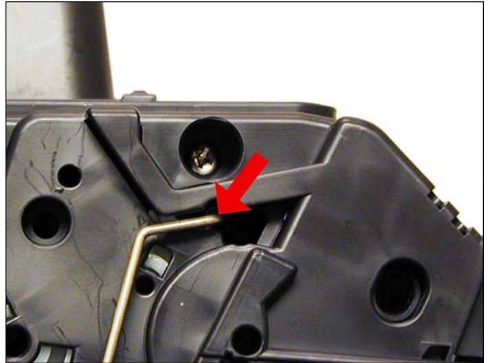
43. Install the metal bars from the drum cover on both sides of the cartridge.
